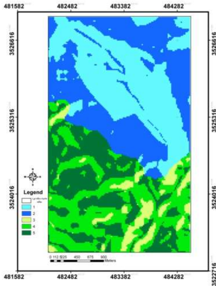
Figure 2: the maps of suitable area for coppice regeneration
