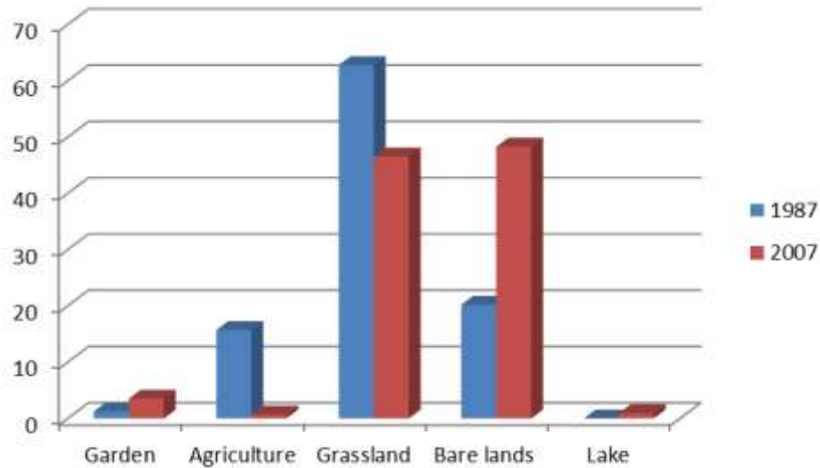
Figure 6: Percentage of plant covers in year 1987 and 2007 year
