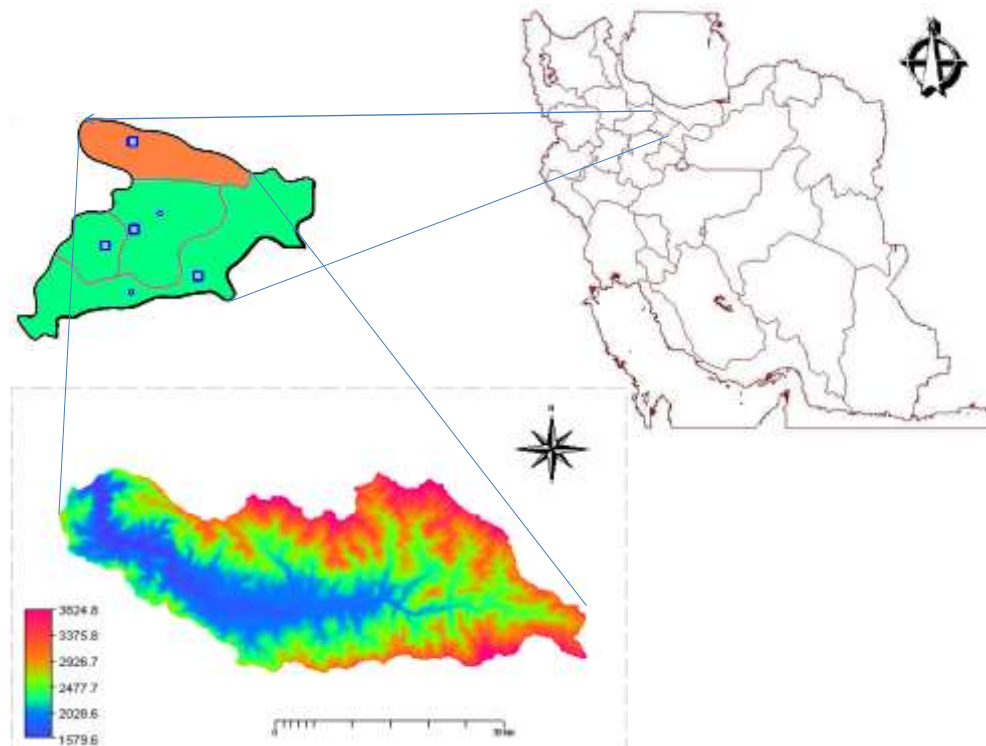
Figure 2: Position of Taleghan area in Iran and its digital elevation model
