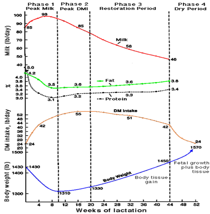
Fig. 1. variations of milk factors in dairy cattle during one lactation period.
