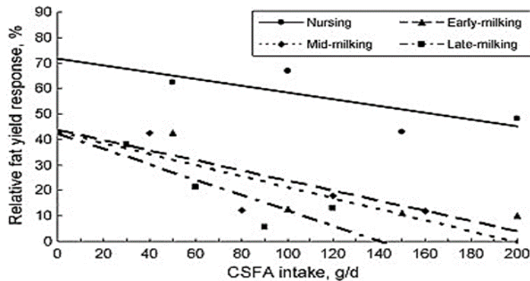
Fig. 2. Relation between intake CSFA and fat yield response in dairy ewes.
